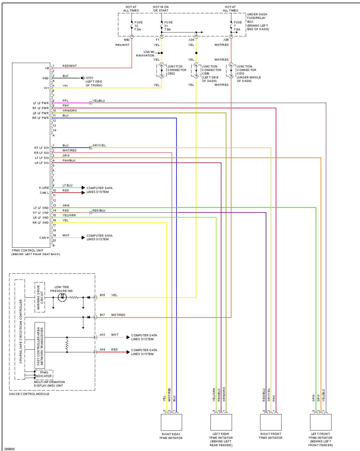
Fig. 103: Tire Pressure Monitoring Circuit
