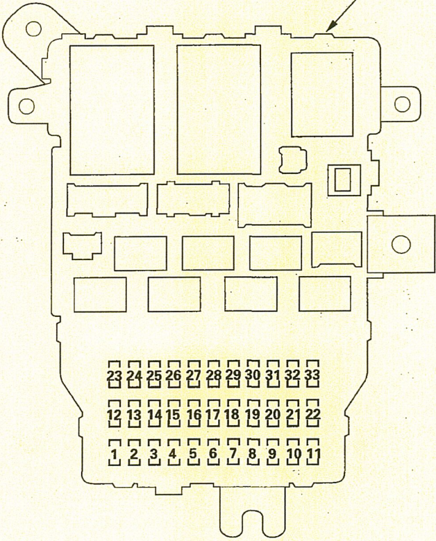
UNDER-DASH FUSE/RELAY BOX
