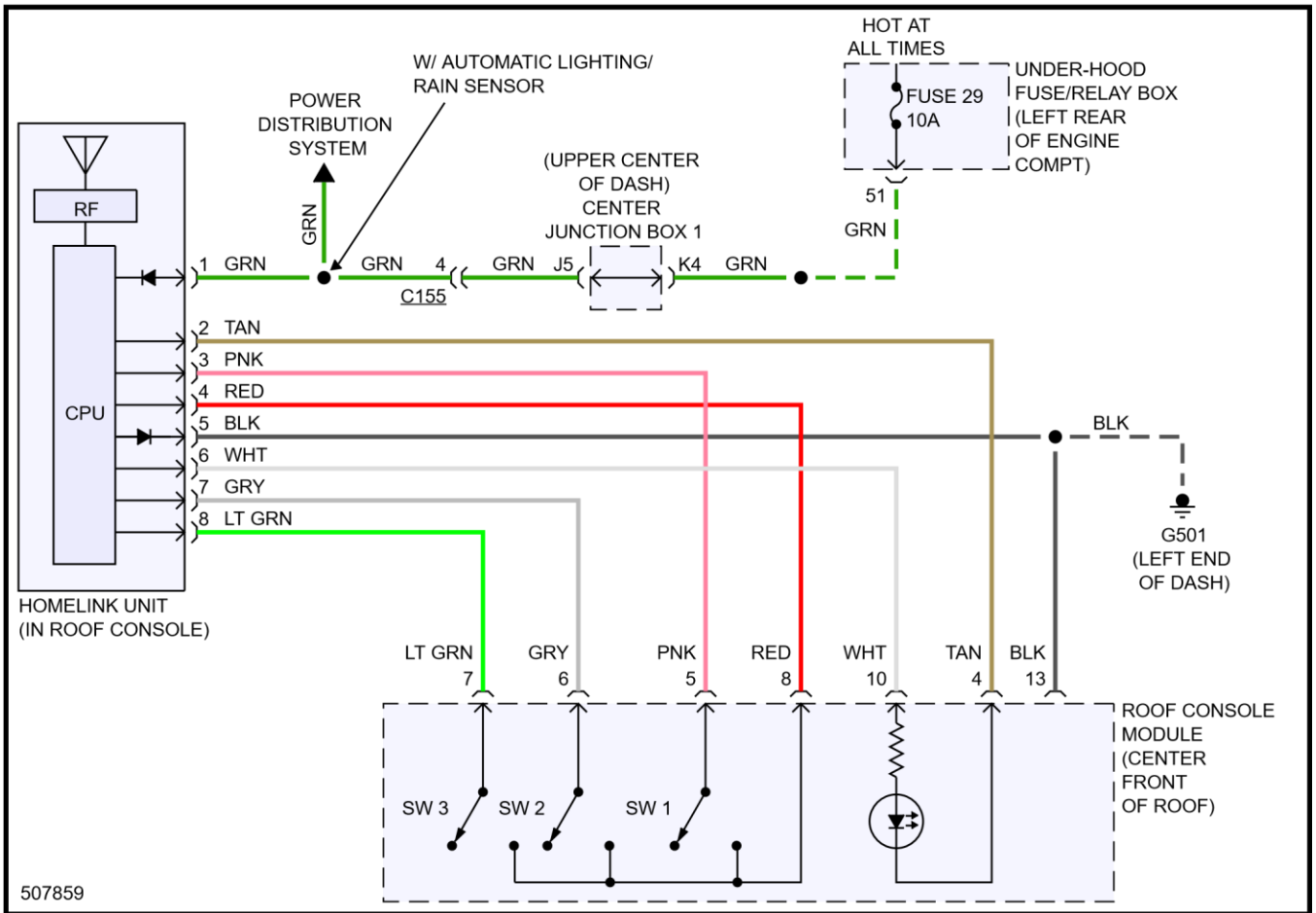
Fig 4: Lane Departure Warning Circuit
