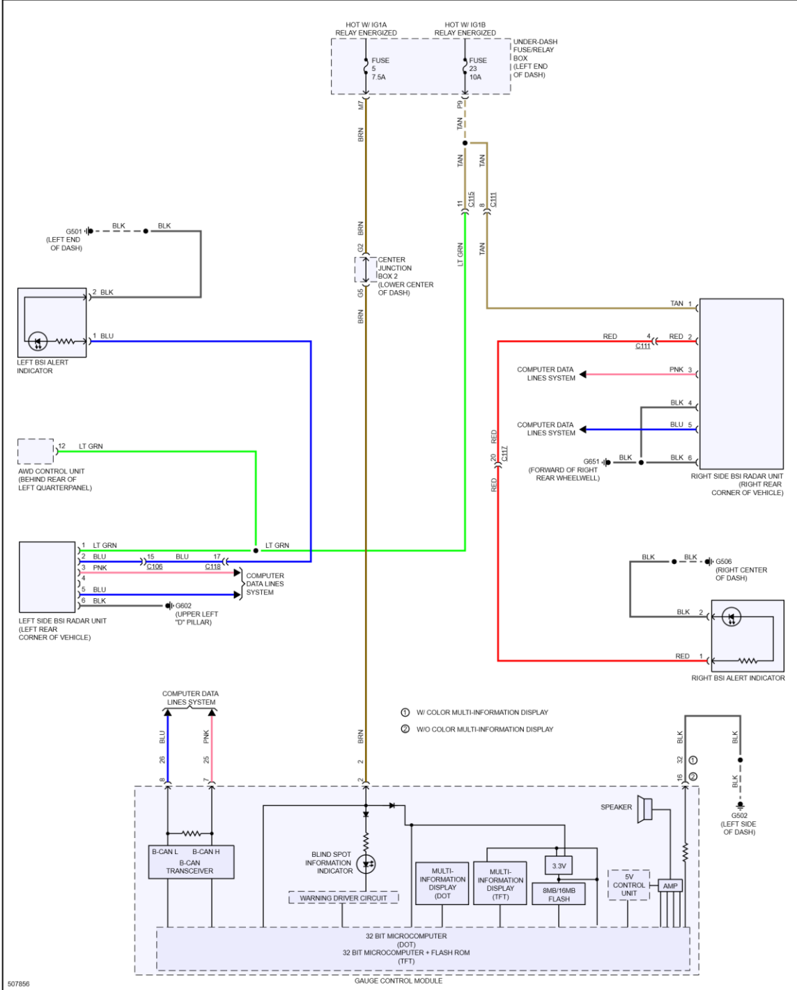
Fig 2: Compass Circuit
