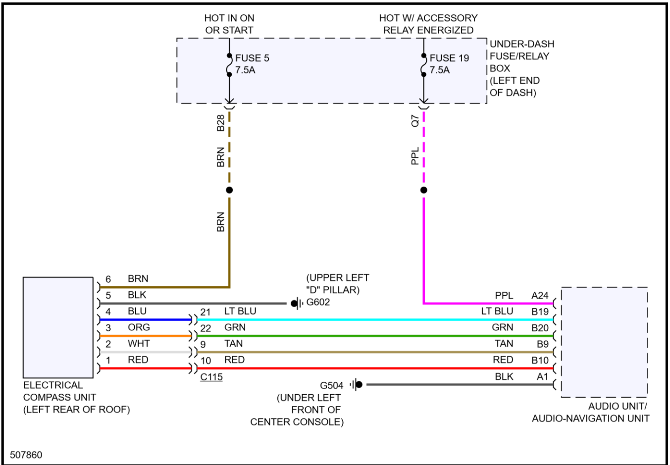
Fig 3: Home Link Remote Control Circuit
