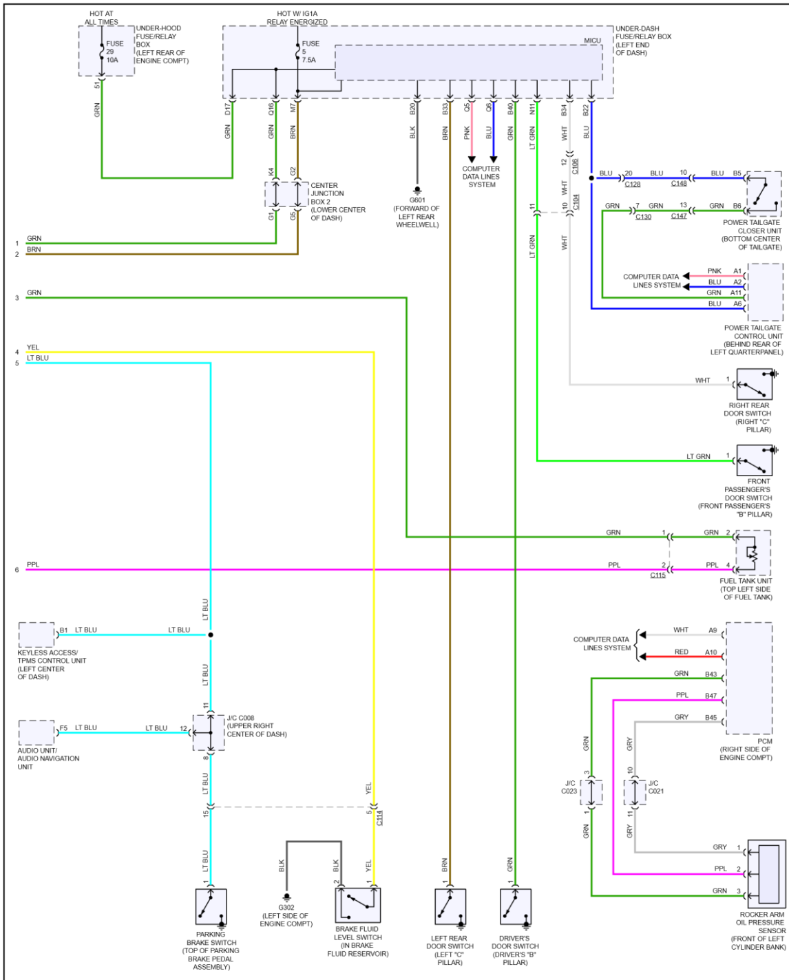
Fig 3: Instrument Cluster Circuit, W/O Color Display (1 of 2)
