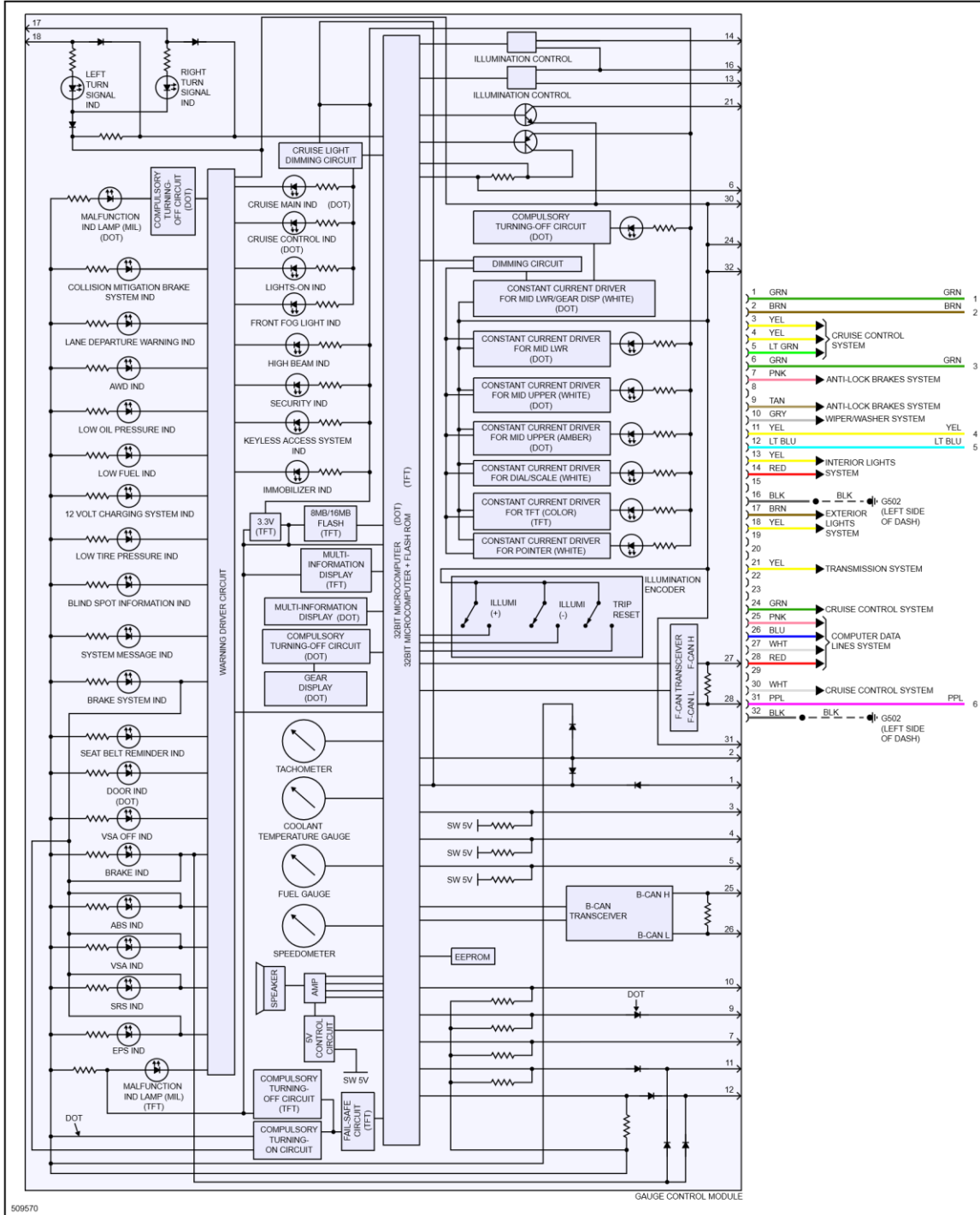
Fig 2: Instrument Cluster Circuit, W/ Color Display (2 of 2)
