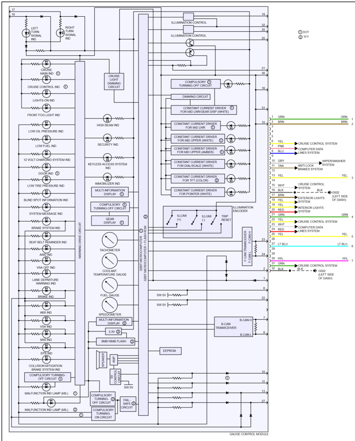
Fig 4: Instrument Cluster Circuit, W/O Color Display (2 of 2)
