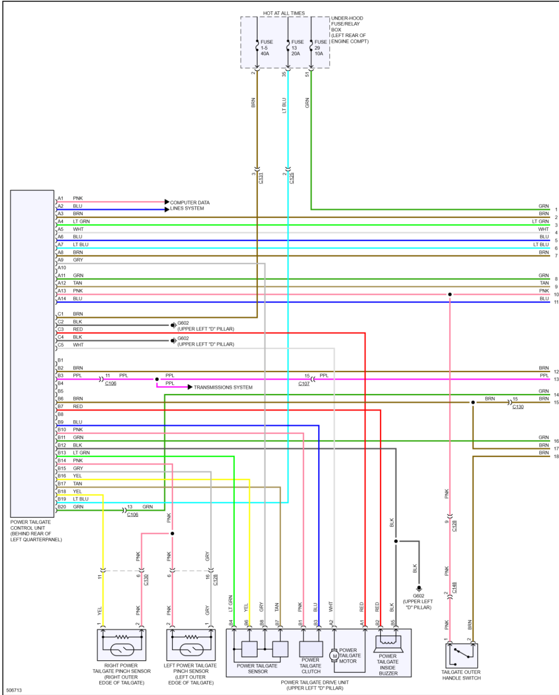
Fig 2: Power Tailgate Circuit (2 of 2)
