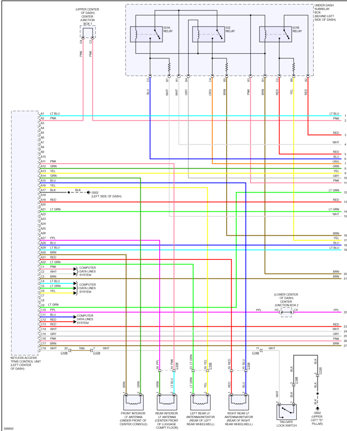
Fig 2: Power Door Locks Circuit (2 of 6)
