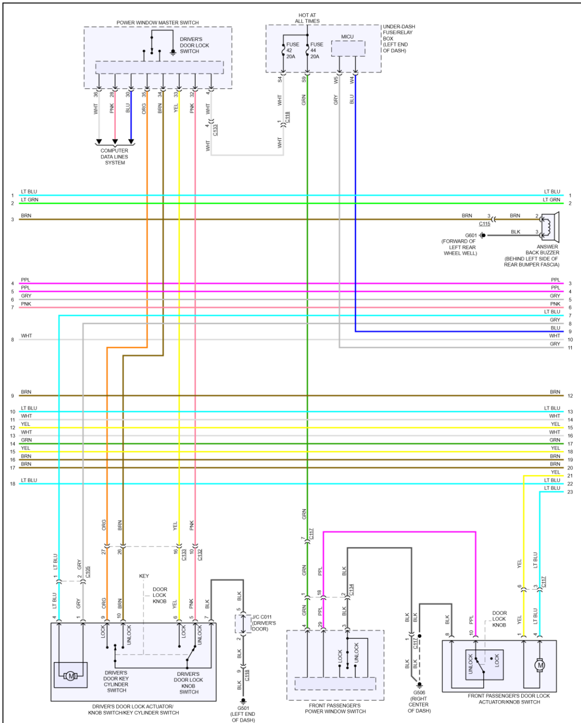
Fig 5: Power Door Locks Circuit (5 of 6)
