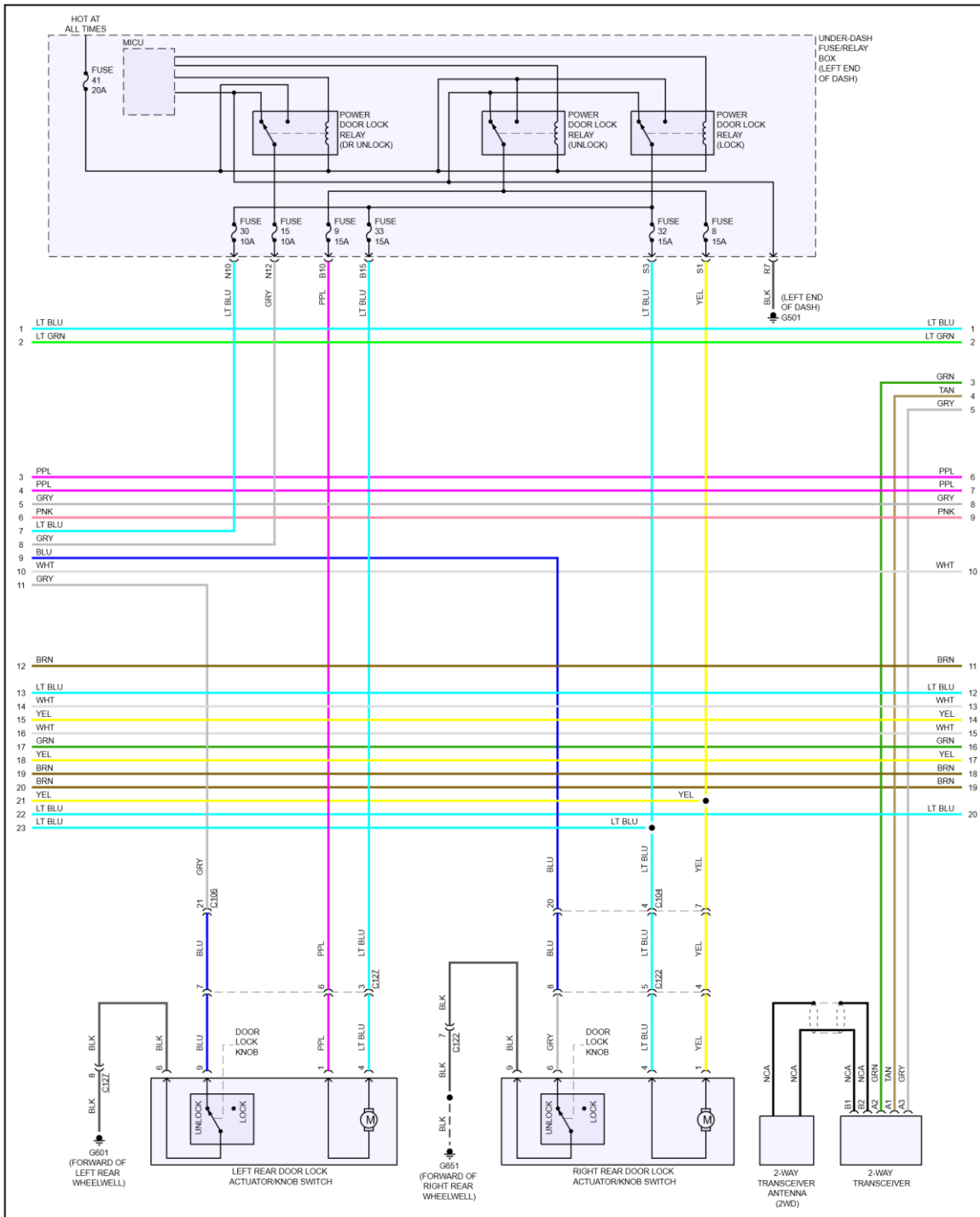
Fig 6: Power Door Locks Circuit (6 of 6)
