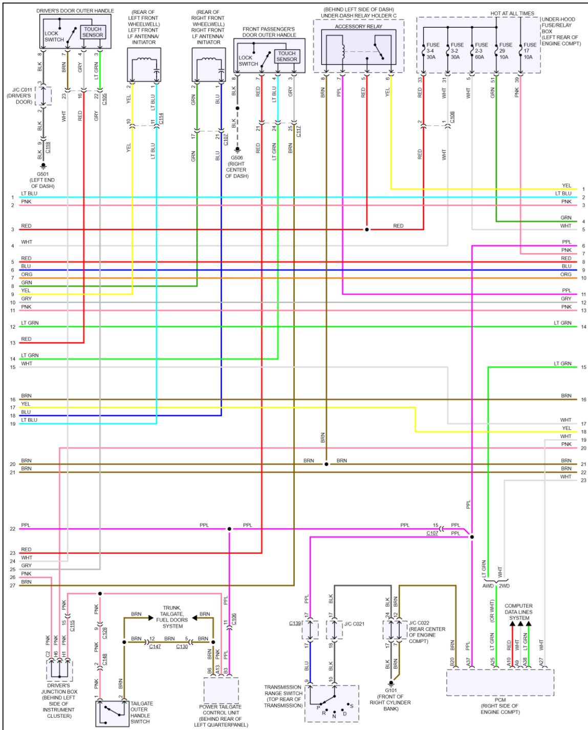
Fig 3: Power Door Locks Circuit (3 of 6)
