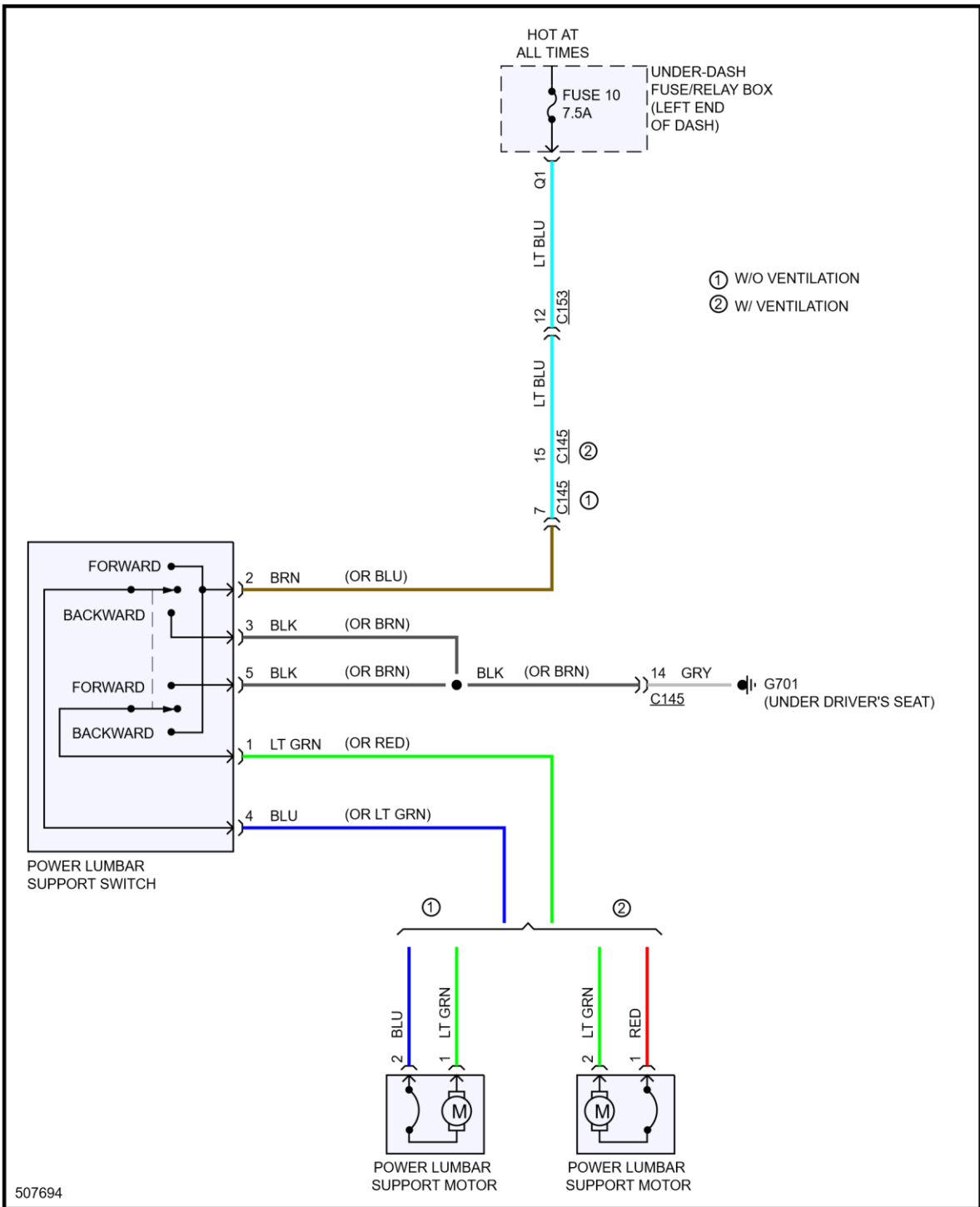
Fig 3: Passenger Power Seat Circuit, 4-Way
