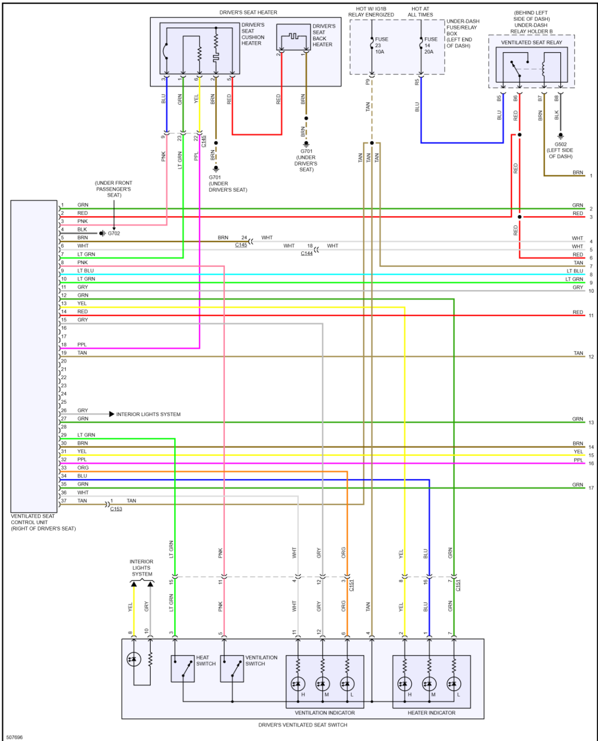
Fig 7: Seat Ventilation Circuit (2 of 2)
