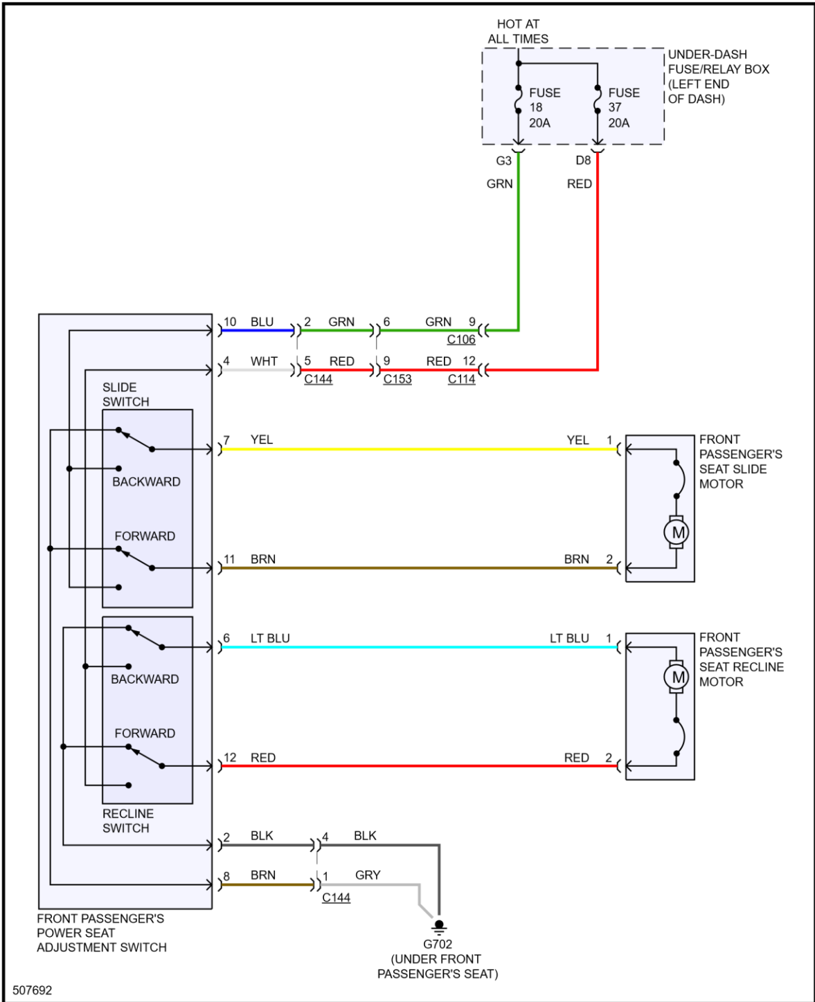
Fig 4: Passenger Power Seat Circuit, 8-Way
