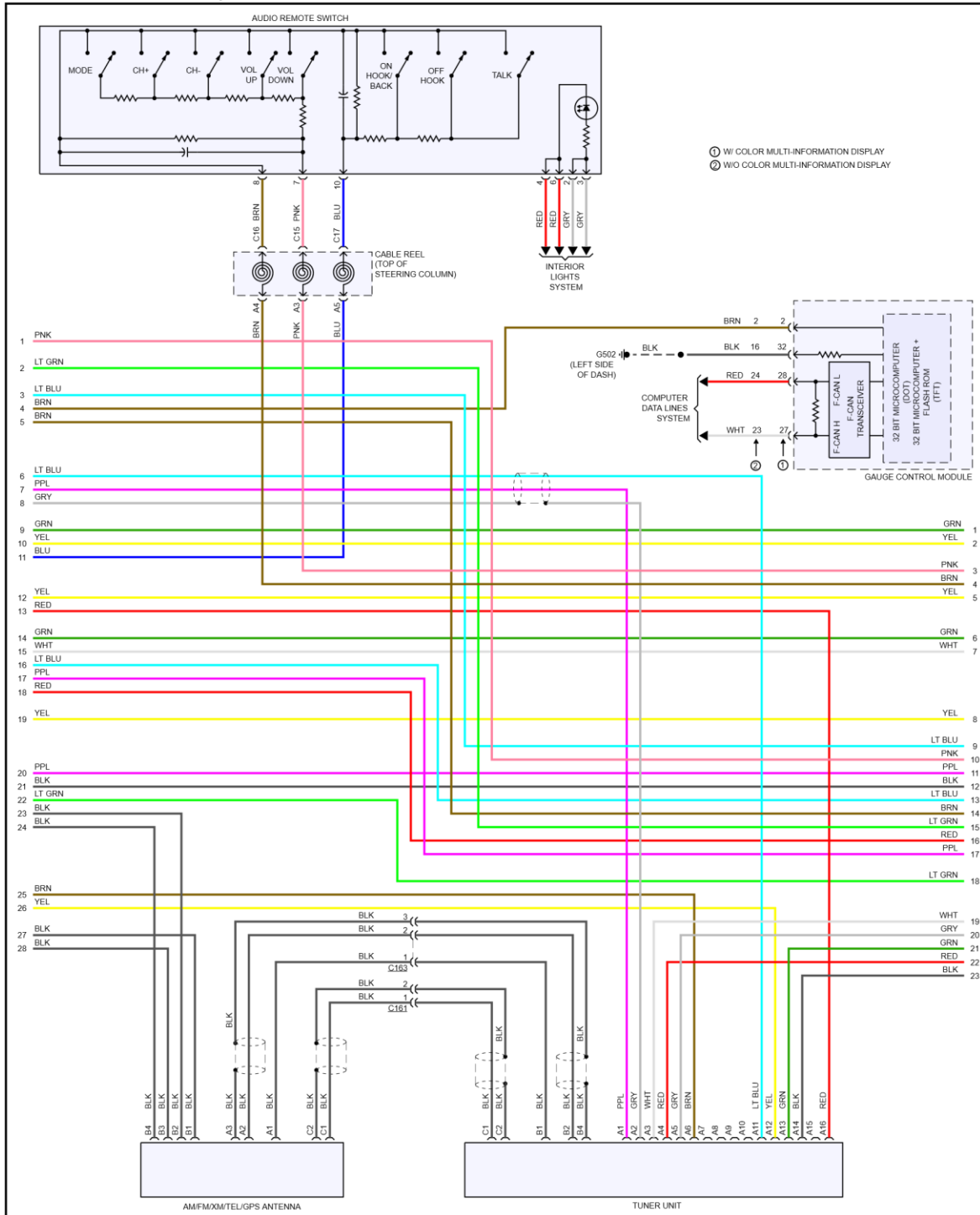
Fig 4: Radio Circuit, W/ Navigation (4 of 5)
