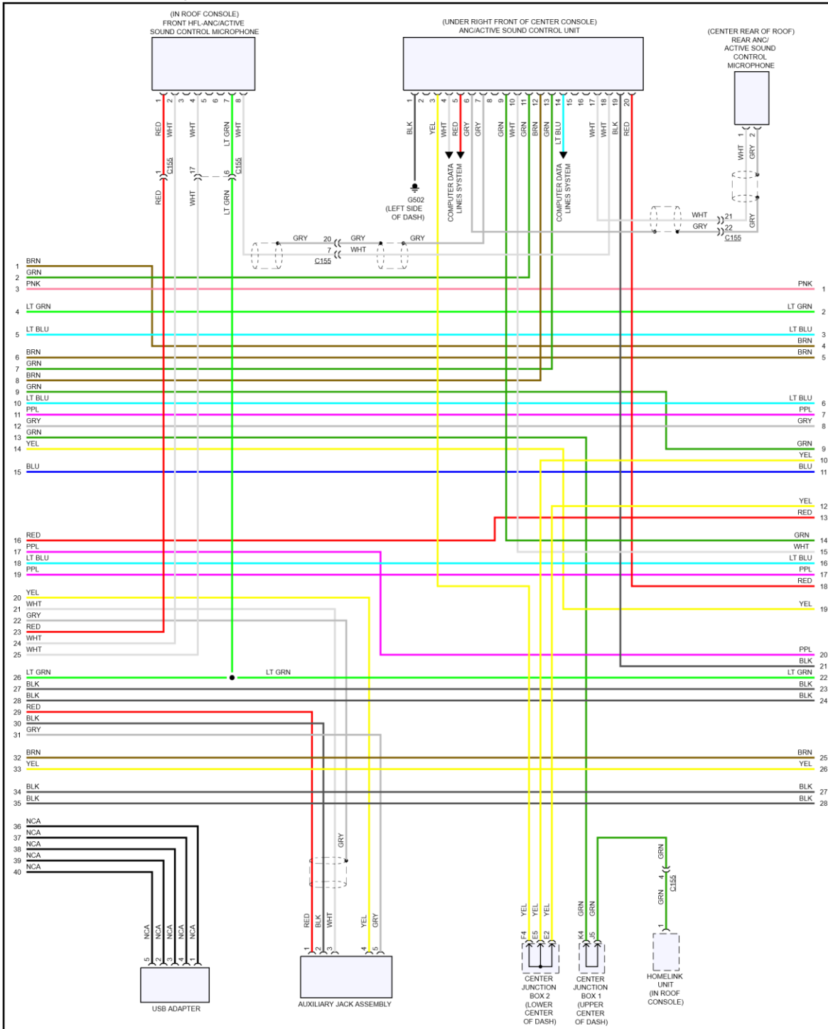
Fig 3: Radio Circuit, W/ Navigation (3 of 5)
