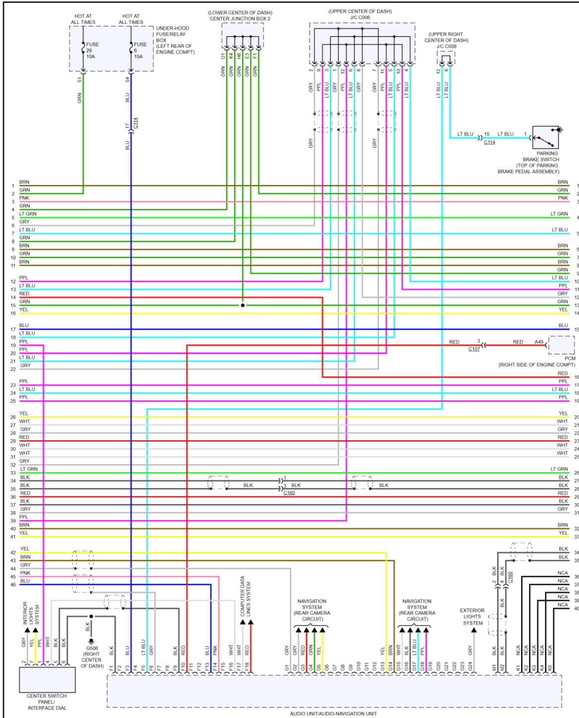
Fig 2: Radio Circuit, W/ Navigation (2 of 5)
