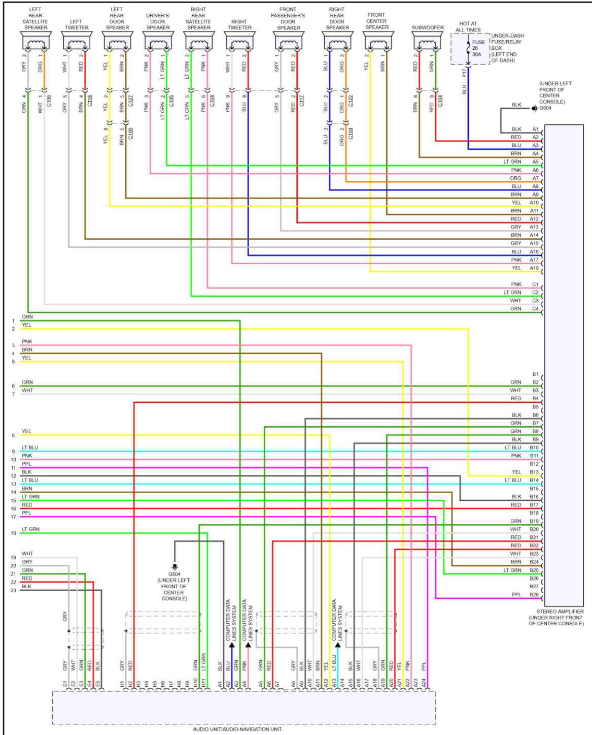
Fig 5: Radio Circuit, W/ Navigation (5 of 5)
