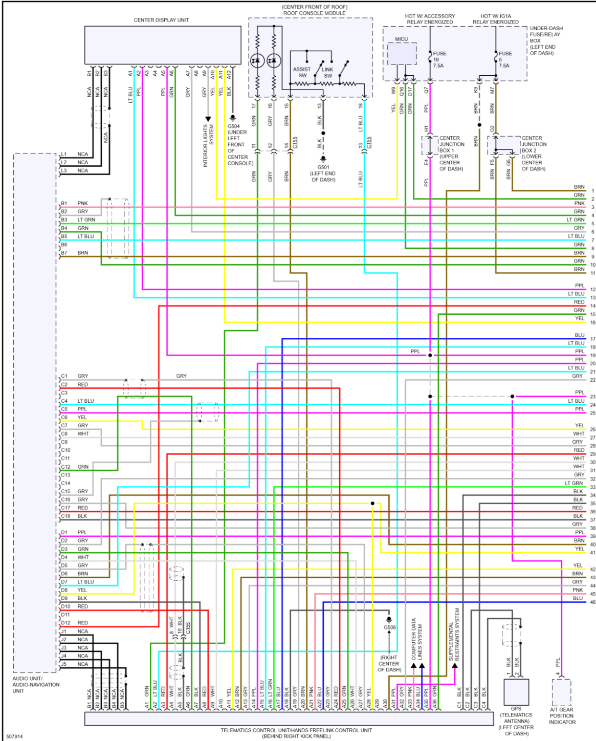
Fig 1: Radio Circuit, W/ Navigation (1 of 5)
