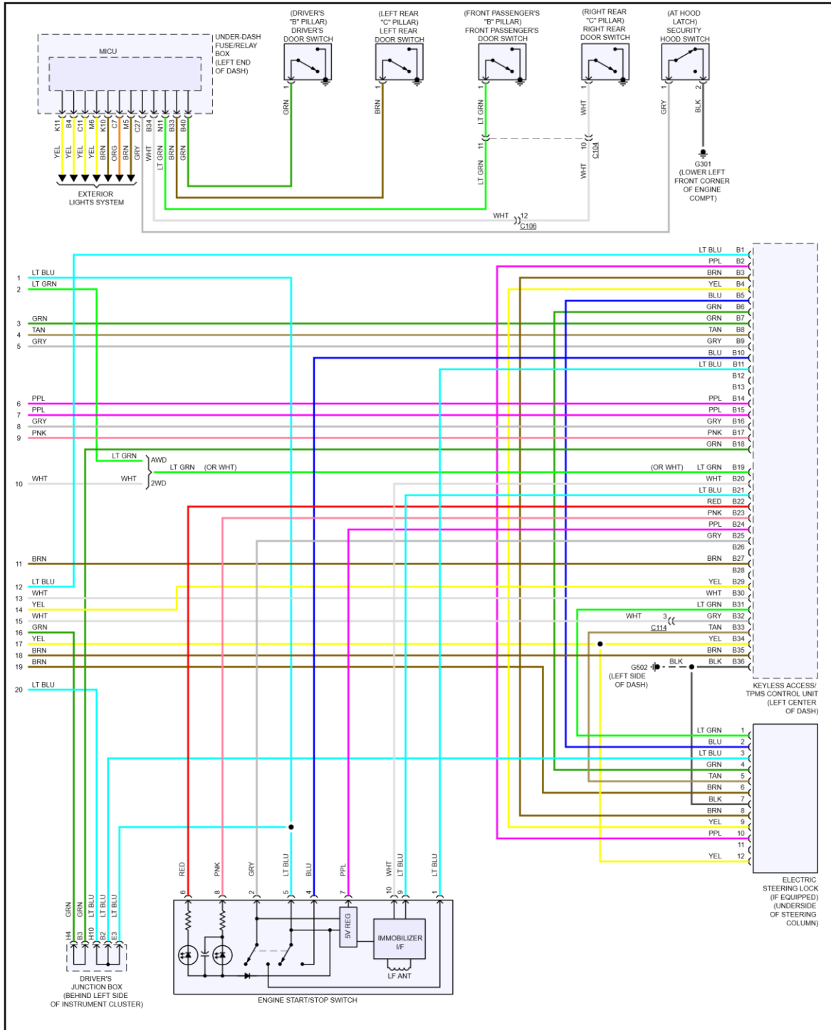
Fig 6: Anti-theft Circuit (6 of 6)
