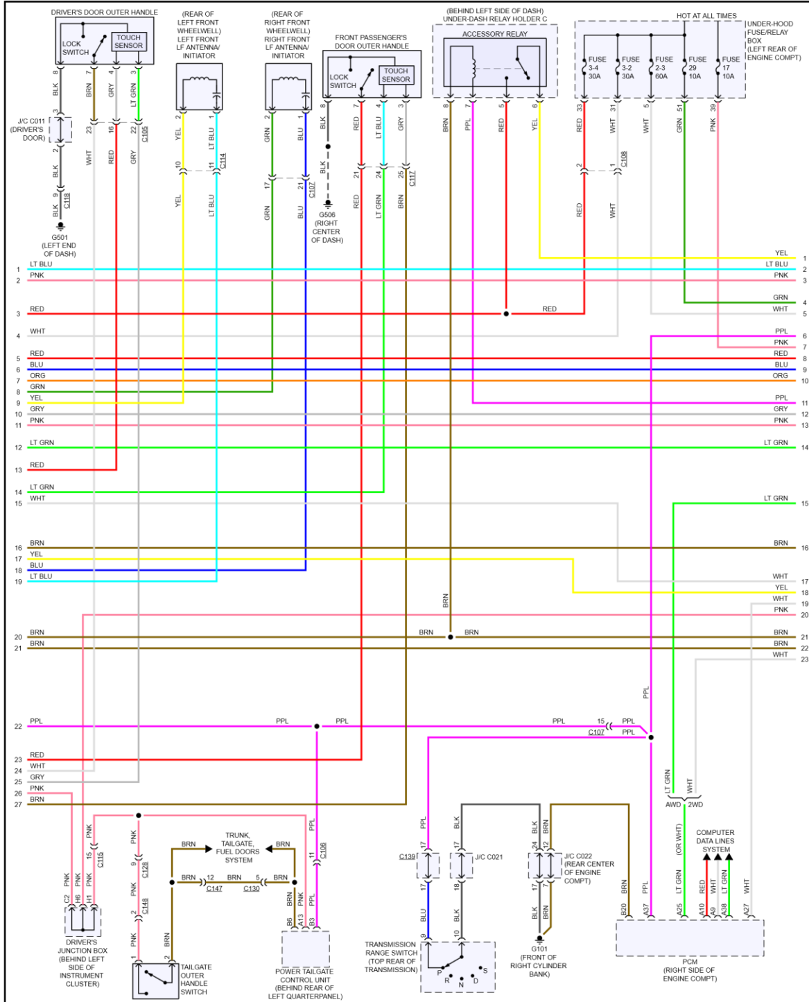
Fig 2: Anti-theft Circuit (2 of 6)
