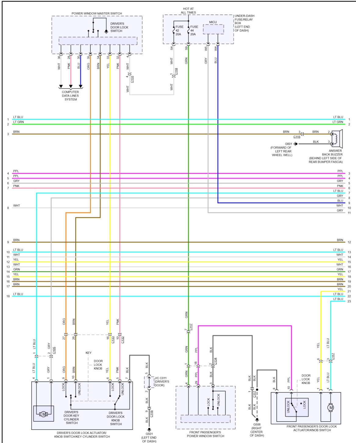
Fig 4: Anti-theft Circuit (4 of 6)
