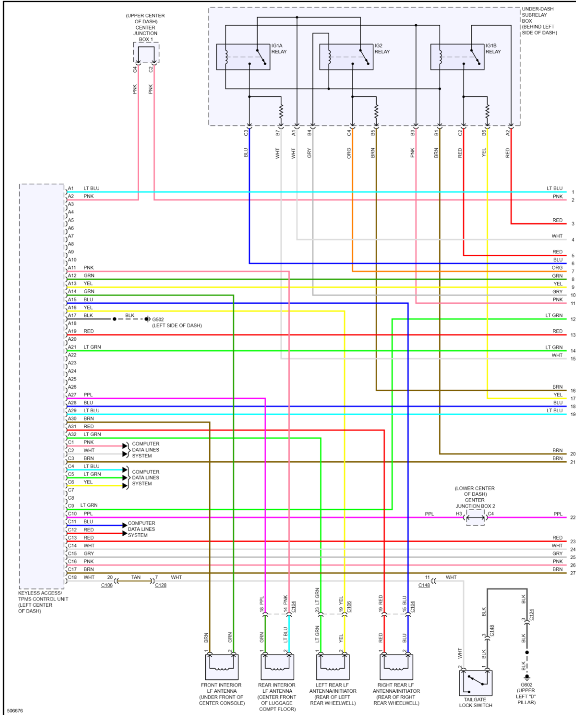
Fig 1: Anti-theft Circuit (1 of 6)
