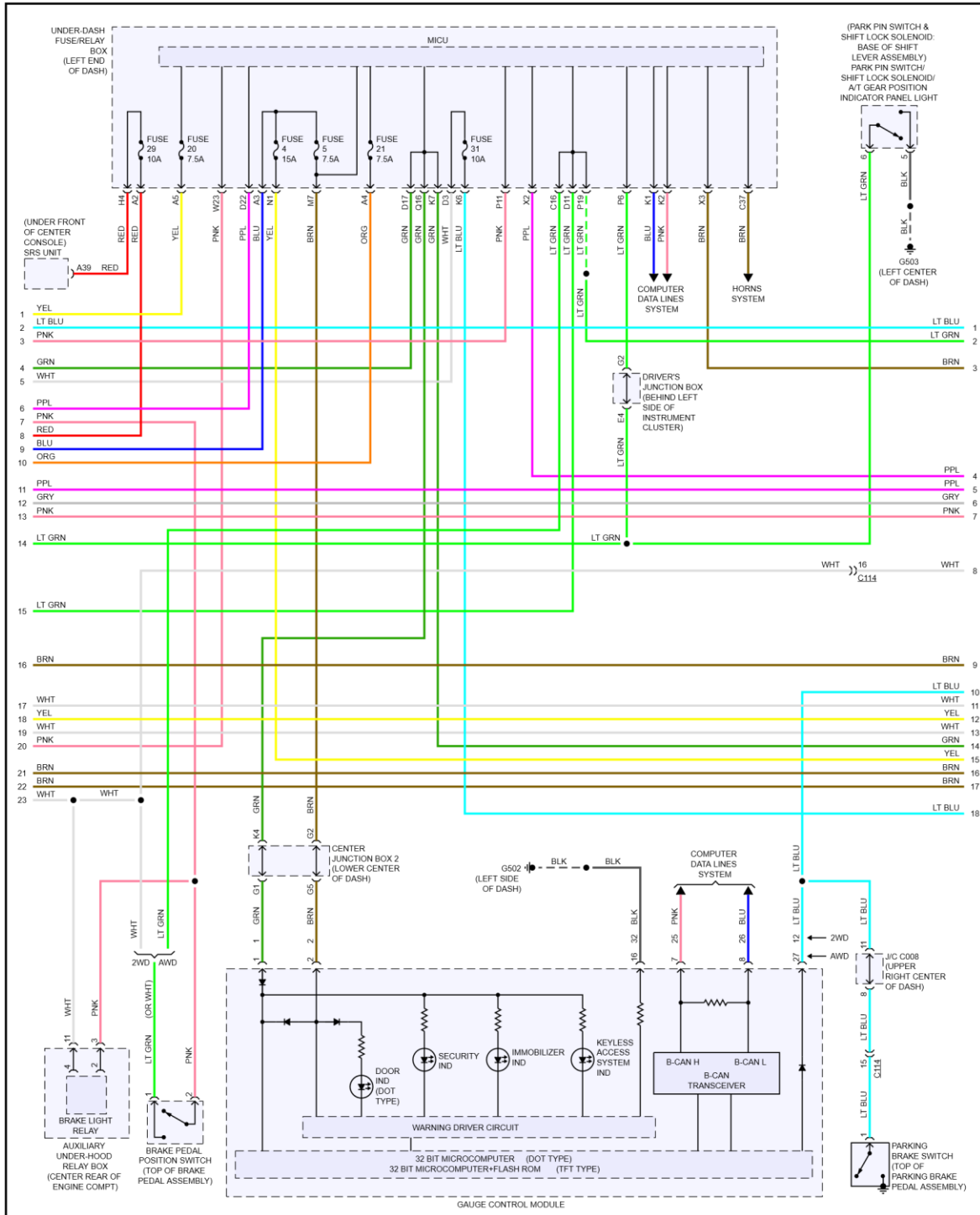
Fig 3: Anti-theft Circuit (3 of 6)
